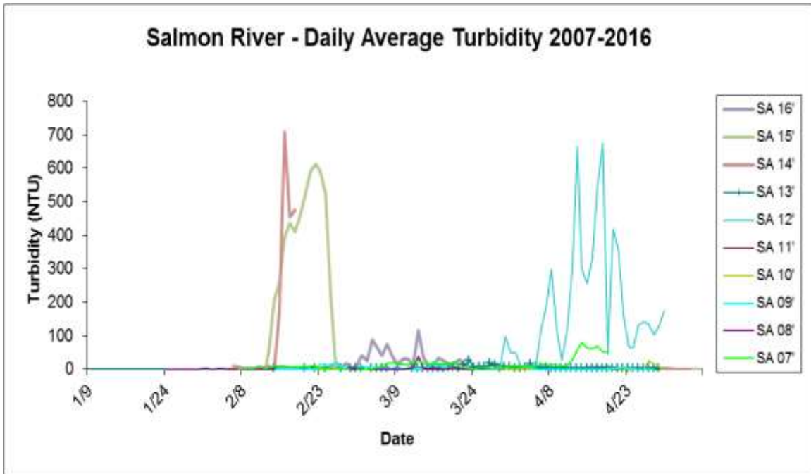
Figure 32. Daily average turbidity, winters of 2007 - 2016 on Salmon River (SA).
