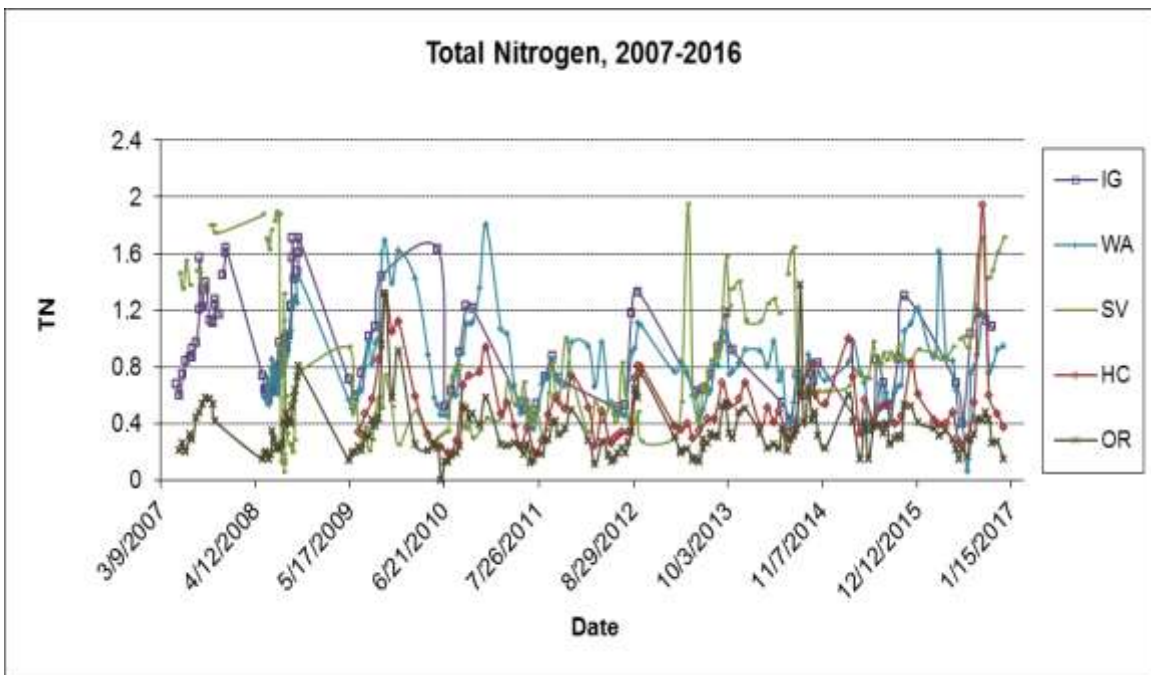
Figure 38. Total Nitrogen measured in mg/L for Klamath River during 2007-2016.
