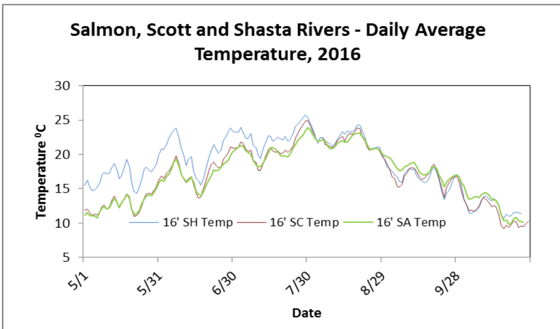
Figure 14. Daily average water temperature for Scott, Shasta, and Salmon Rivers, 2016.
