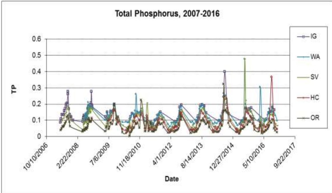
Figure 35. Total Phosphorus measured in mg/L for Klamath River sites during 2007-2016.
