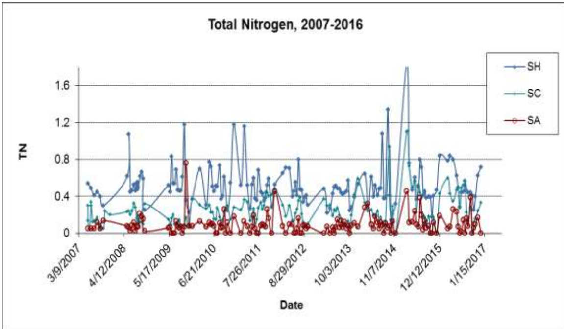
Figure 37. Total Nitrogen measured in mg/L for Salmon, Scott and Shasta Rivers during 2007-2016.
