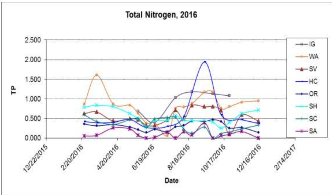
Figure 36. Total Nitrogen measured in mg/L for all monitored sites during 2016.
