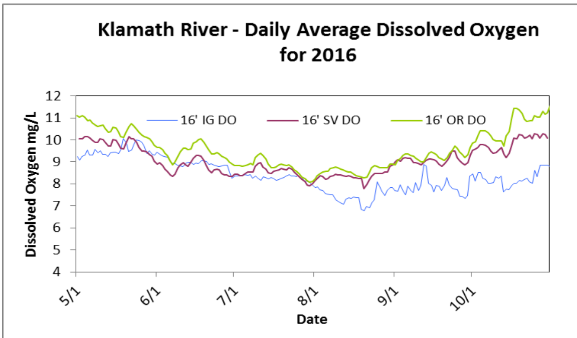
Figure 4. Daily average dissolved oxygen levels for 3 main stem Klamath River sites in 2016: below Iron Gate dam (IG), Seiad Valley (SV), and Orleans (OR).
