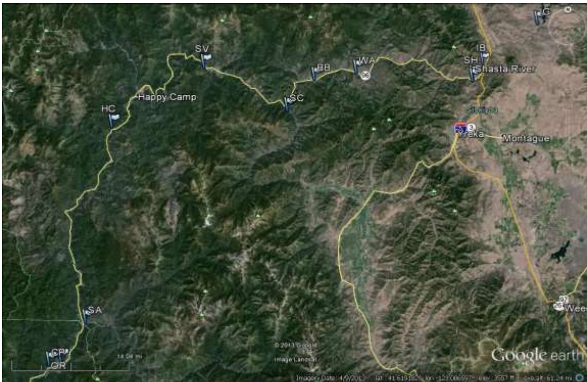
Figure 1. Overview of the Karuk Tribe’s water quality monitoring locations along the Klamath River in 2016.
