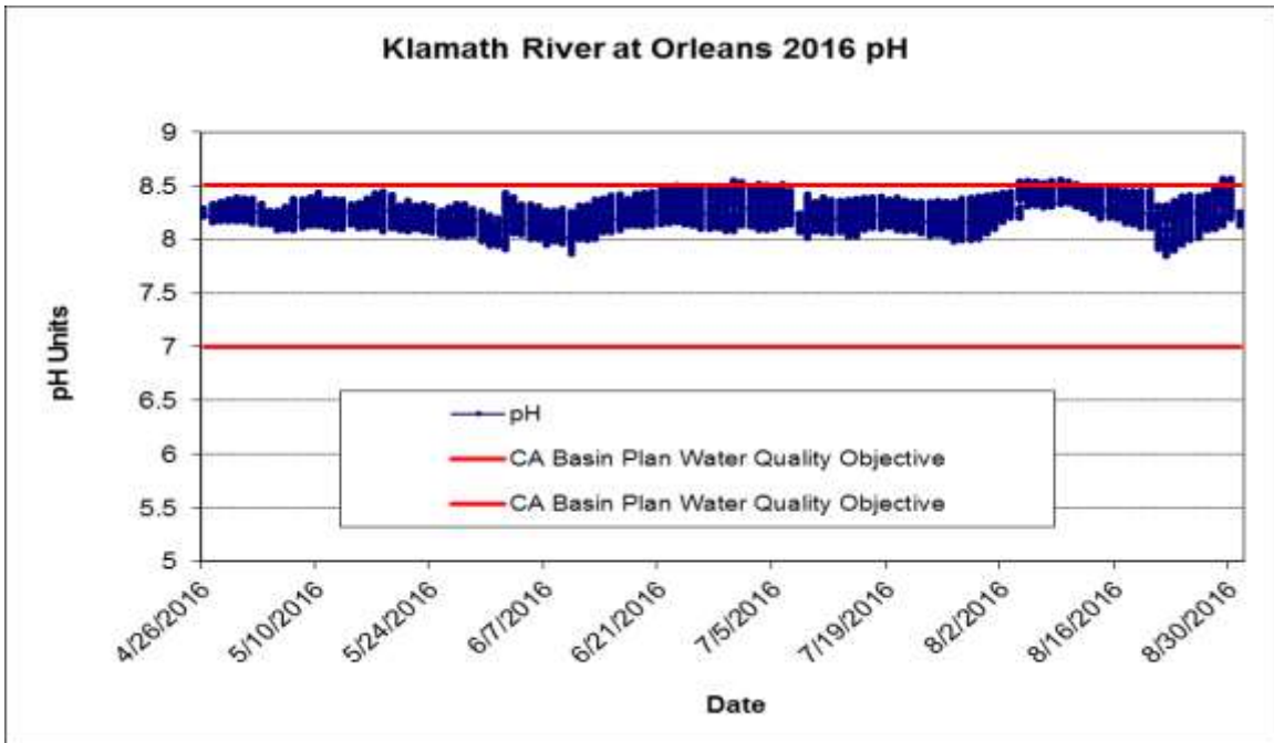
Figure 10. Instantaneous pH readings recorded every 30-minutes for Klamath River at Orleans (OR) in 2016. The red lines are the NCRWQCB Basin Plan water quality objectives for the Klamath River, 7 < X < 8.5 .
