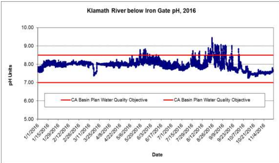
Figure 12. Instantaneous pH readings recorded every 30-minutes for Klamath River below Iron Gate (IG) in 2016. The red lines are the NCRWQCB Basin Plan water quality objectives for the Klamath River, 7 < X < 8.5
