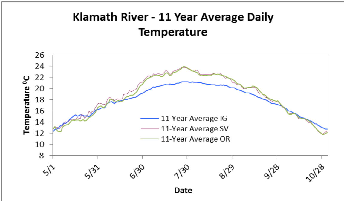
Figure 3. Averaged daily temperature from 2006-2016 at main stem Klamath River sites: below Iron Gate dam (IG), Seiad Valley (SV), and Orleans (OR).
