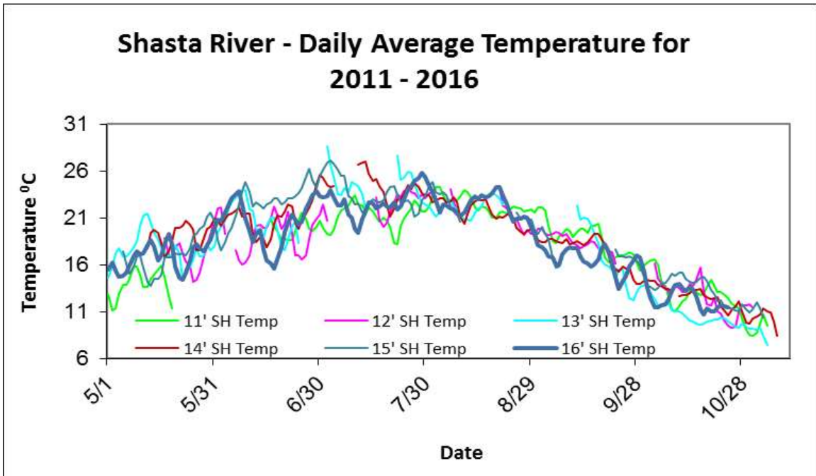
Figure 15. Daily average water temperatures for the Shasta River from 2011-2016.
