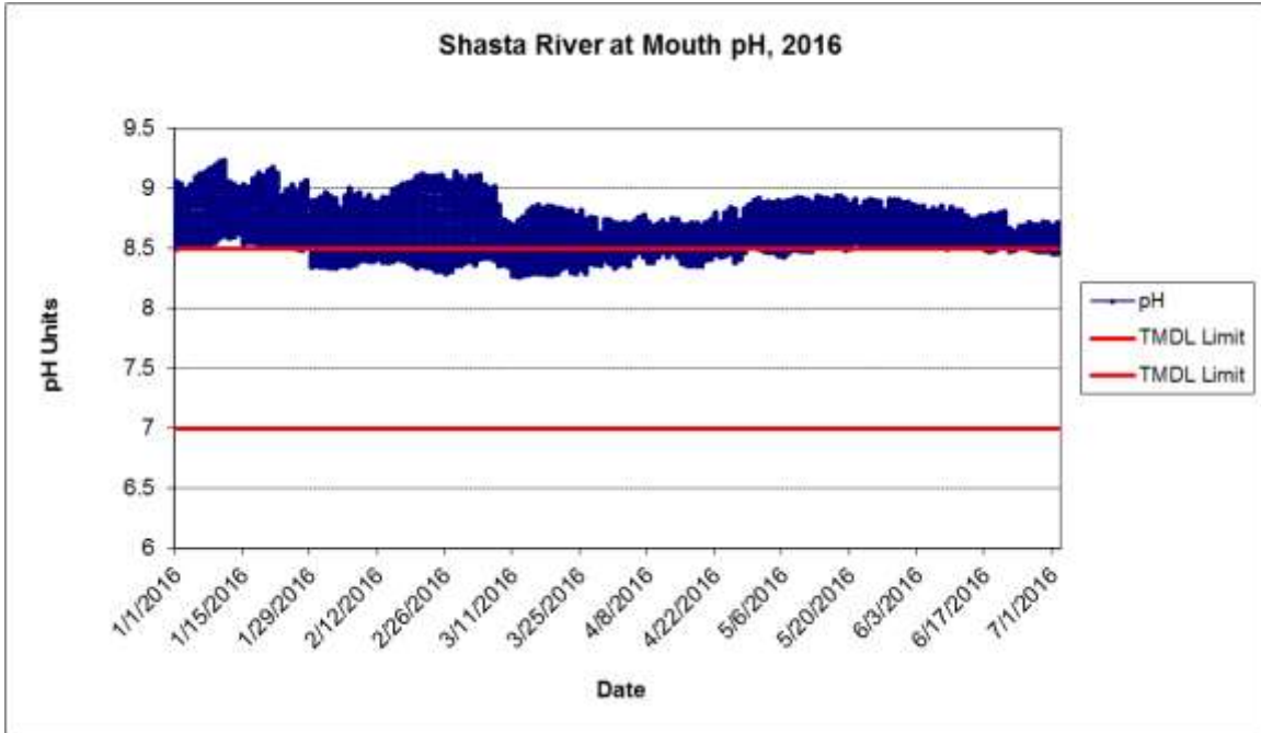
Figure 27. Instantaneous pH readings recorded every 30 minutes for the mouth of the Shasta River (SH) in 2016. The red line indicates the NCRWQCB Basin Plan pH water quality objective for Shasta River, 7 < X < 8.5 .
