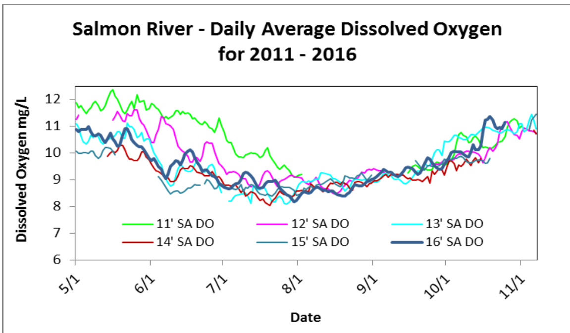
Figure 23. Daily average dissolved oxygen concentrations for the Salmon River from 2011-2016.
