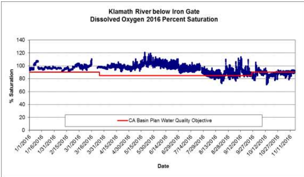
Figure 7. Percent saturation dissolved oxygen readings recorded every 30-minutes for Klamath River below Iron Gate Dam (IG) in 2016. The red line indicates the NCRWQCB Basin Plan Klamath River site specific dissolved oxygen water quality objective from Stateline (OR/CA) to the mouth of the Scott River, >90% saturation from Oct 1- March 30 and >85% from April 1-Sept 30.
