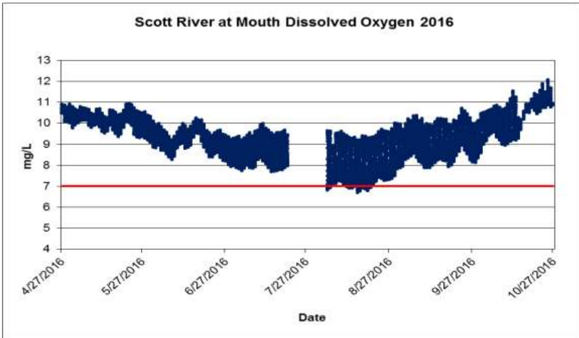
Figure 22. Instantaneous dissolved oxygen readings recorded every 30-minutes for the mouth of the Scott River (SC) in 2016. The red line indicates the NCRWQCB Basin Plan site specific dissolved oxygen water quality objective for Scott River, >7mg/L.
