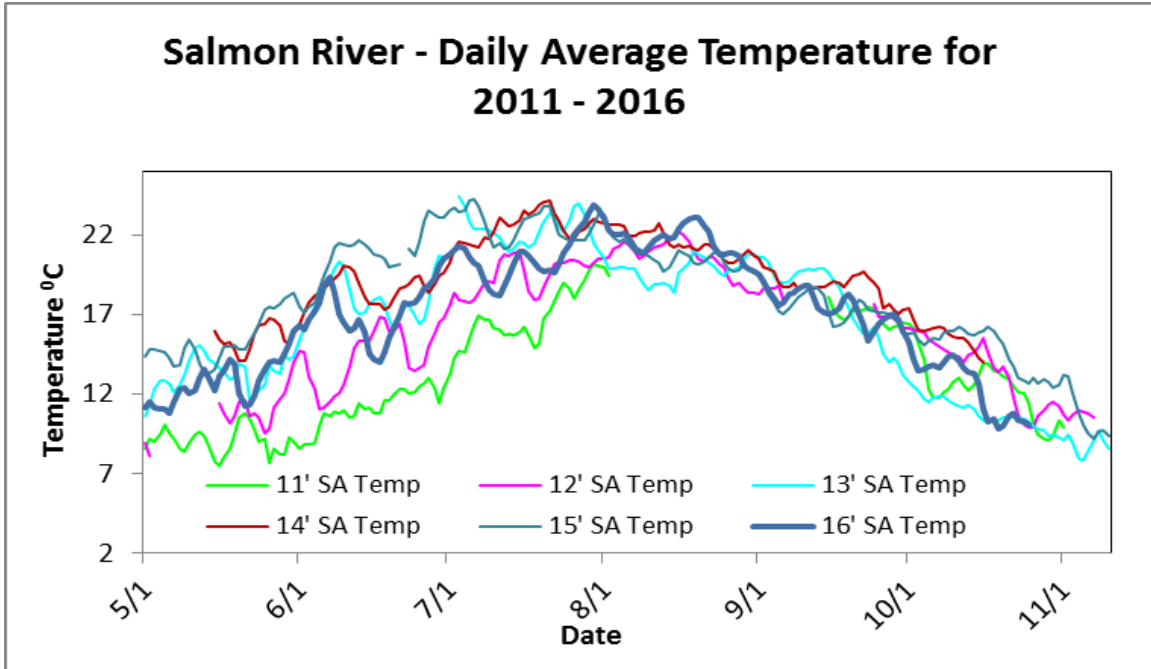
Figure 17. Daily average water temperatures for the Salmon River from 2011-2016.
