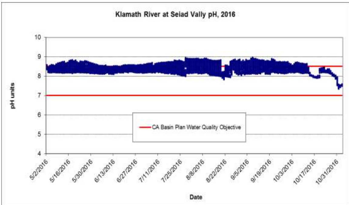
Figure 11. Instantaneous pH readings recorded every 30-minutes for Klamath River below Seiad Valley (SV) in 2016. The red lines are the NCRWQCB Basin Plan water quality objectives for the Klamath River, 7 < X < 8.5
