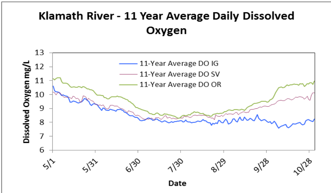
Figure 8. Average daily dissolved oxygen levels from 2006-2016 at main stem Klamath River sites: below Iron Gate dam (IG), Seiad Valley (SV), and Orleans (OR).
