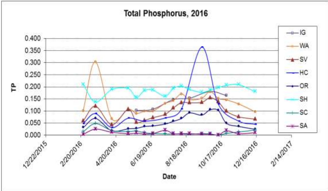
Figure 33. Total Phosphorus measured in mg/L for all monitored sites during 2016.
