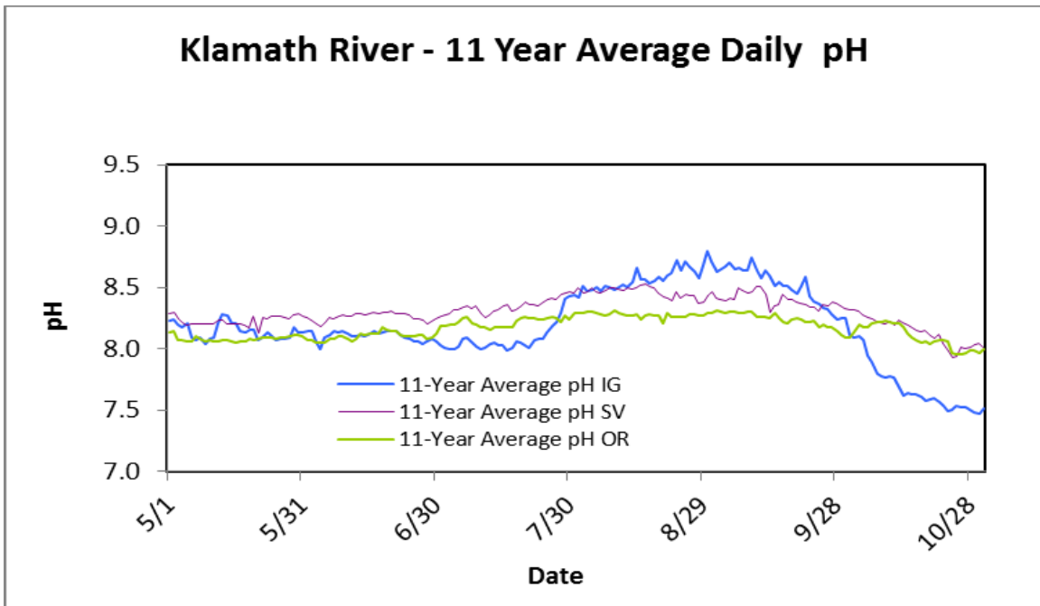
Figure 13. Daily average pH, 2006-2016 at main stem Klamath River sites: below Iron Gate dam (IG), Seiad Valley (SV), and Orleans (OR).
