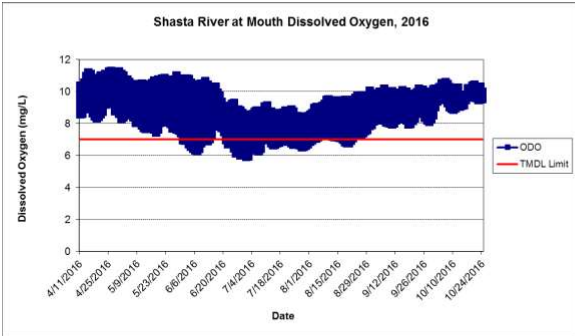
Figure 20. Instantaneous dissolved oxygen recorded every 30-minutes for the mouth of the Shasta River (SH) in 2016. The red line indicates the NCRWQCB Basin Plan site specific dissolved oxygen water quality objective for Shasta River, >7mg/L.
