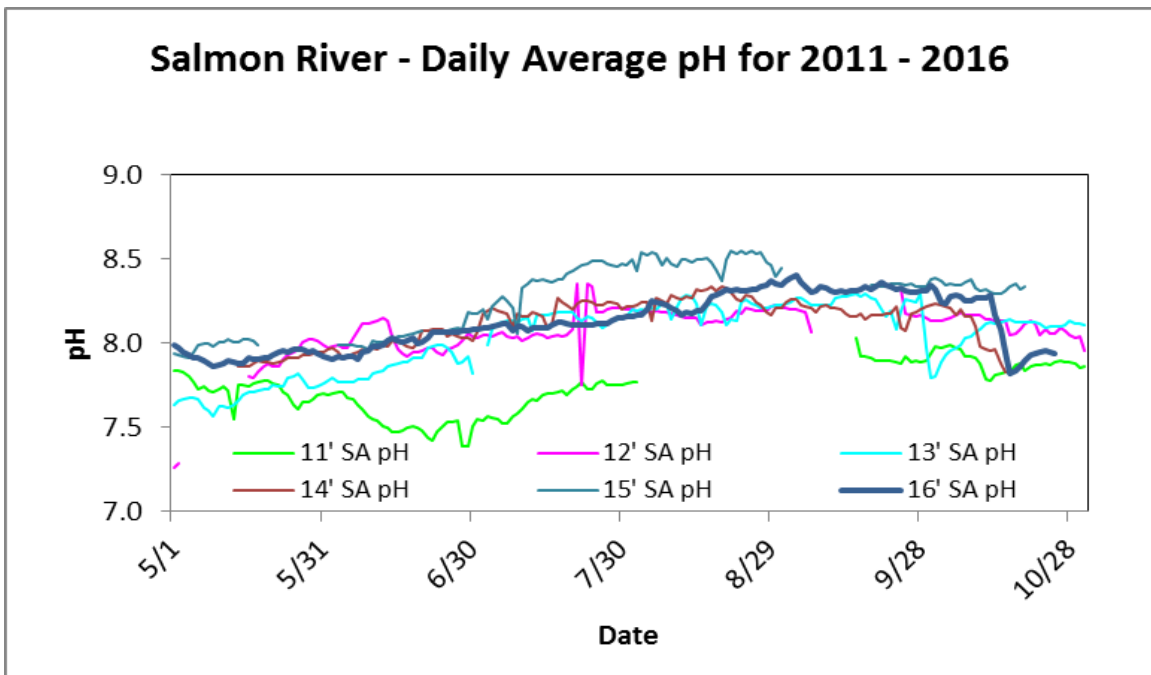
Figure 30. Daily average pH concentrations for the Salmon River from 2011-2016.
