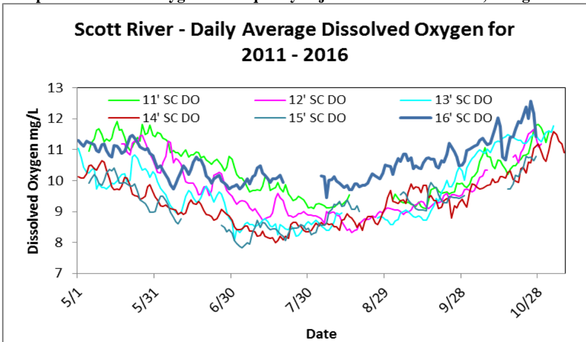
Figure 21. Daily average dissolved oxygen concentrations for the Scott River from 2011-2016.
