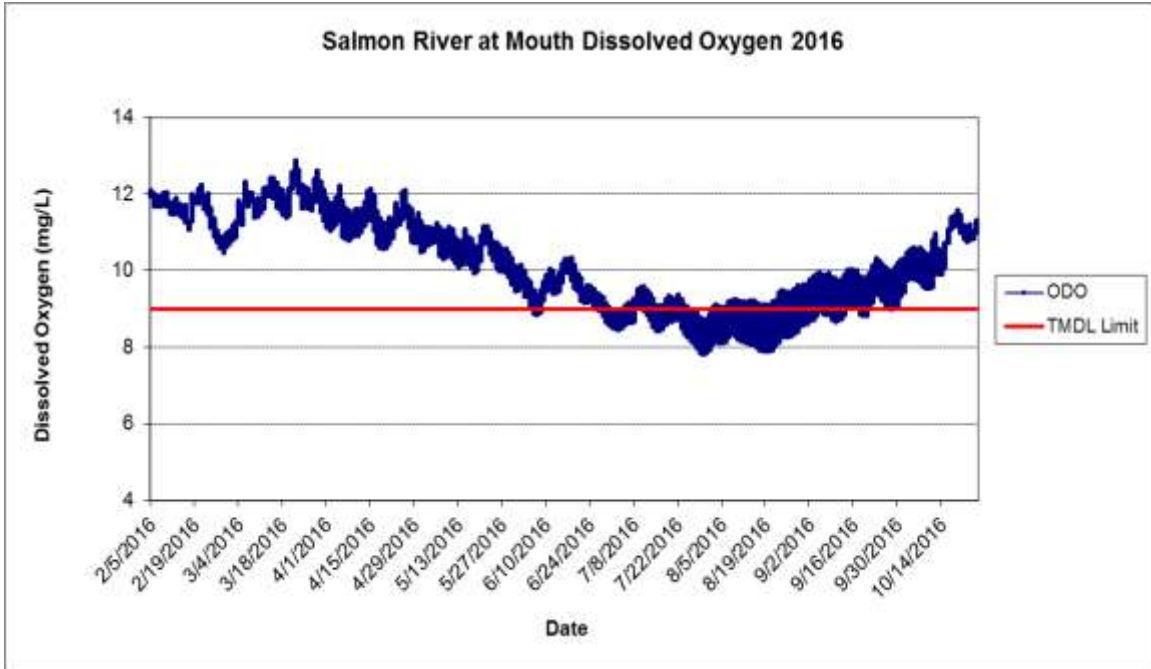
Figure 24: Instantaneous dissolved oxygen readings recorded every 30 minutes for the mouth of the Salmon River (SA) in 2016. The red line indicates the NCRWQCB Basin Plan site specific dissolved oxygen water quality objective for Salmon River, >9mg/L.
