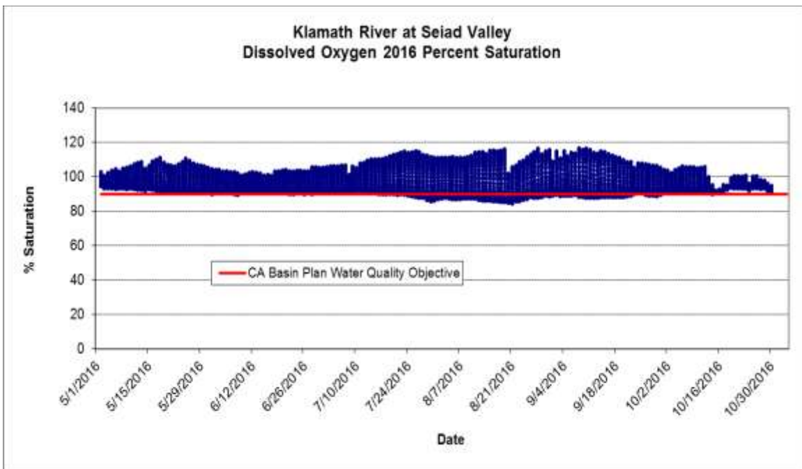
Figure 6. Percent saturation dissolved oxygen readings recorded every 30-minutes for Klamath River at Seiad Valley (SV) in 2016. The red line indicates the NCRWQCB Basin Plan Klamath River site specific dissolved oxygen water quality objective: from the mouth of the Scott River to Hoopa, >90% saturation year-round.
