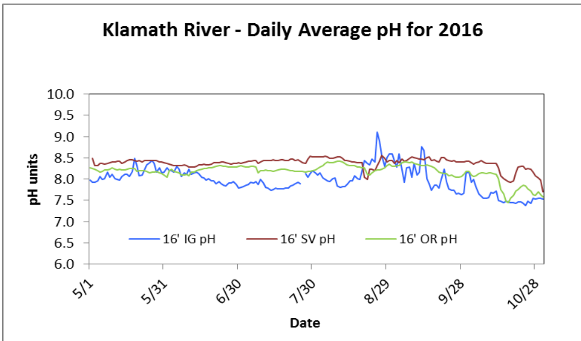
Figure 9. Daily average pH levels for 3 main stem Klamath River sites in 2016: below Iron Gate dam (IG), Seiad Valley (SV), and Orleans (OR).
