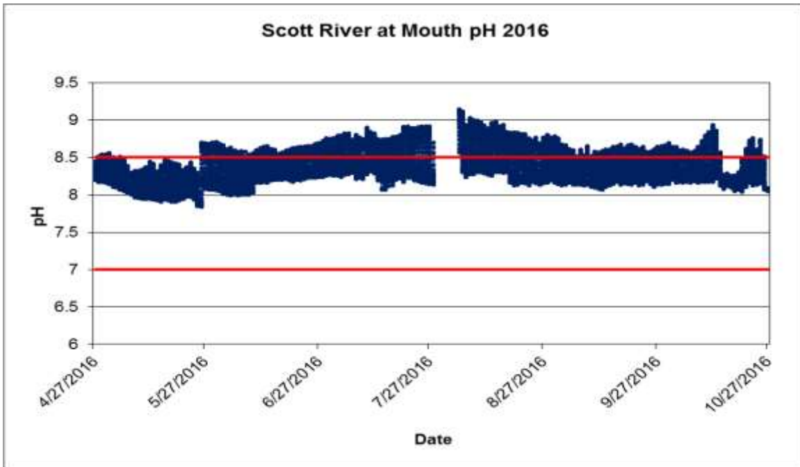
Figure 29. Instantaneous pH readings recorded every 30 minutes for the mouth of the Scott River (SC) in 2016. The red line indicates the NCRWQCB Basin Plan pH water quality objective for Scott River, 7 < X < 8.5 .
