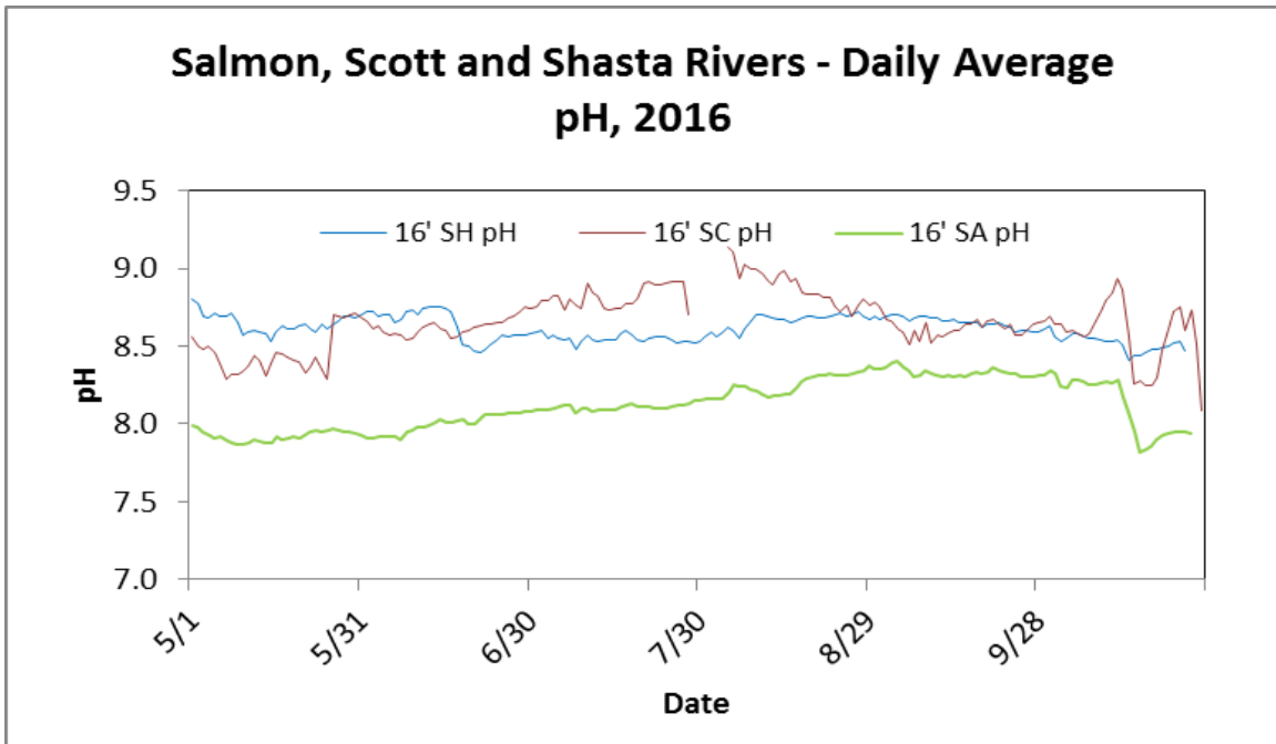
Figure 25. Daily average pH for Scott, Shasta, and Salmon Rivers, 2016.
