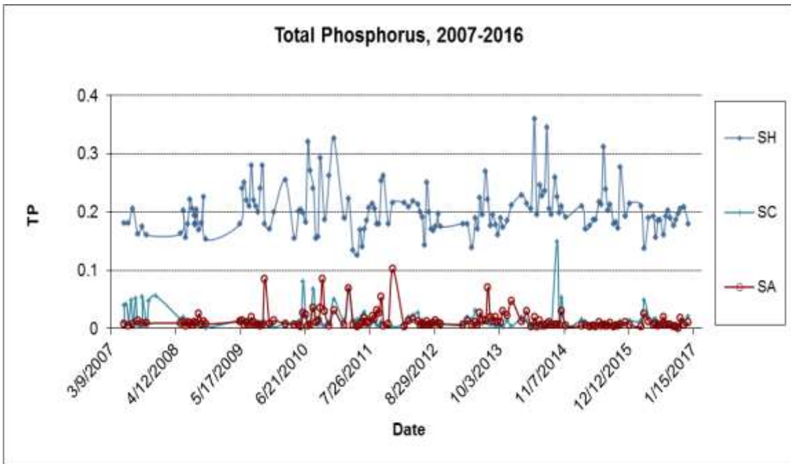
Figure 34. Total Phosphorus measured in mg/L for Salmon, Scott and Shasta Rivers sites during 2007-2016.
