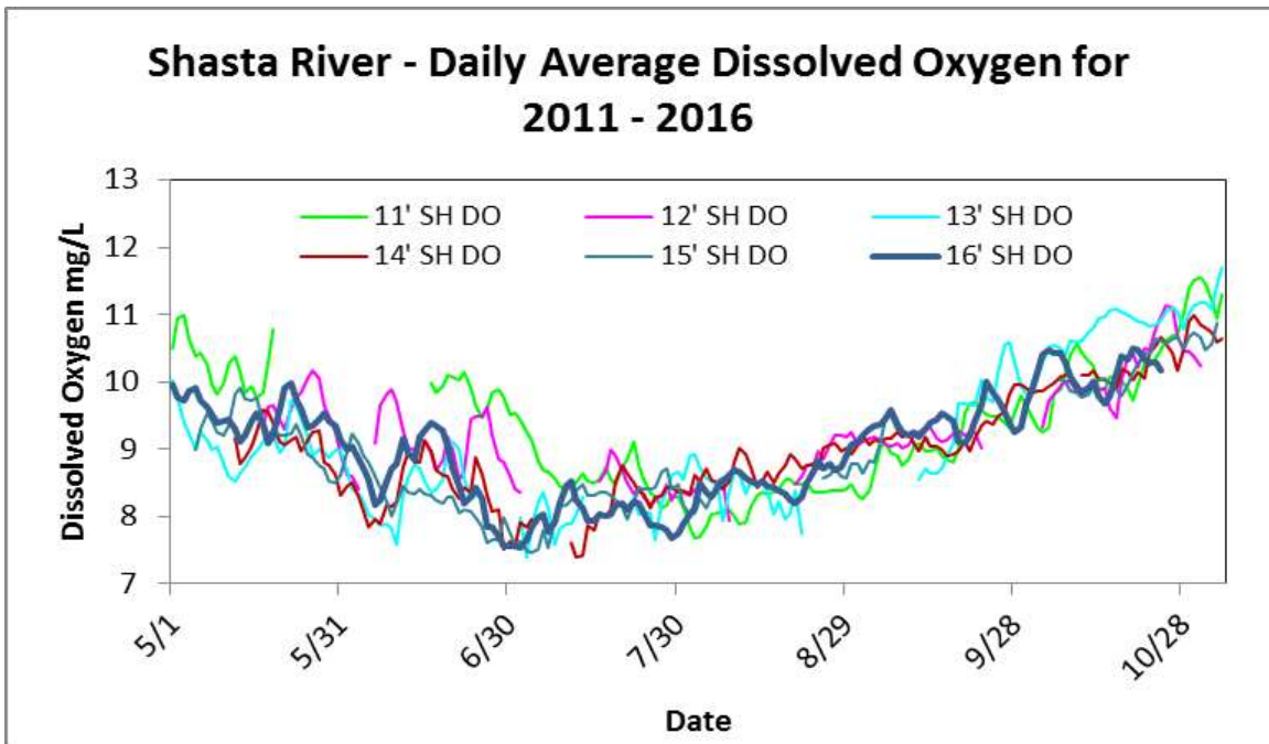
Figure 19. Daily average dissolved oxygen concentrations for the Shasta River from 2011-2016.
