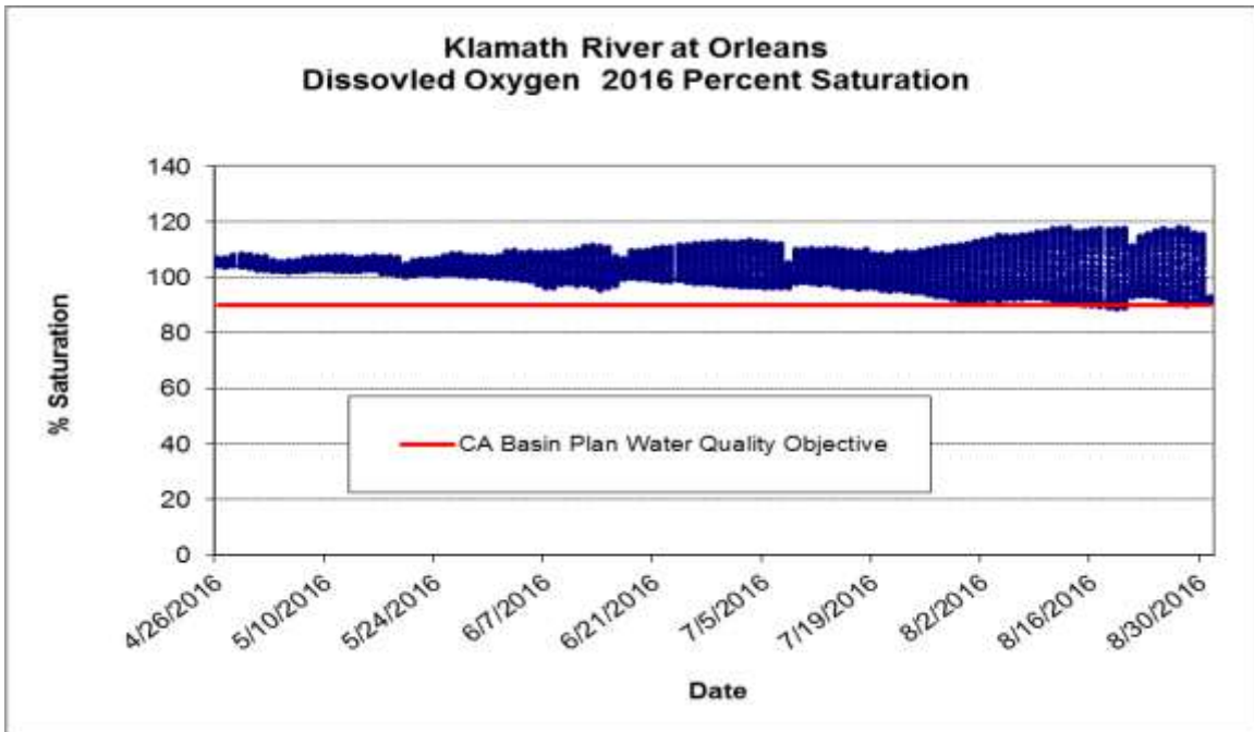
Figure 5. Percent saturation dissolved oxygen readings recorded every 30-minutes for Klamath River at Orleans (OR) in 2016. The red line indicates the NCRWQCB Basin Plan Klamath River site specific dissolved oxygen water quality objective: from the mouth of the Scott River to Hoopa, >90% saturation year-round.
