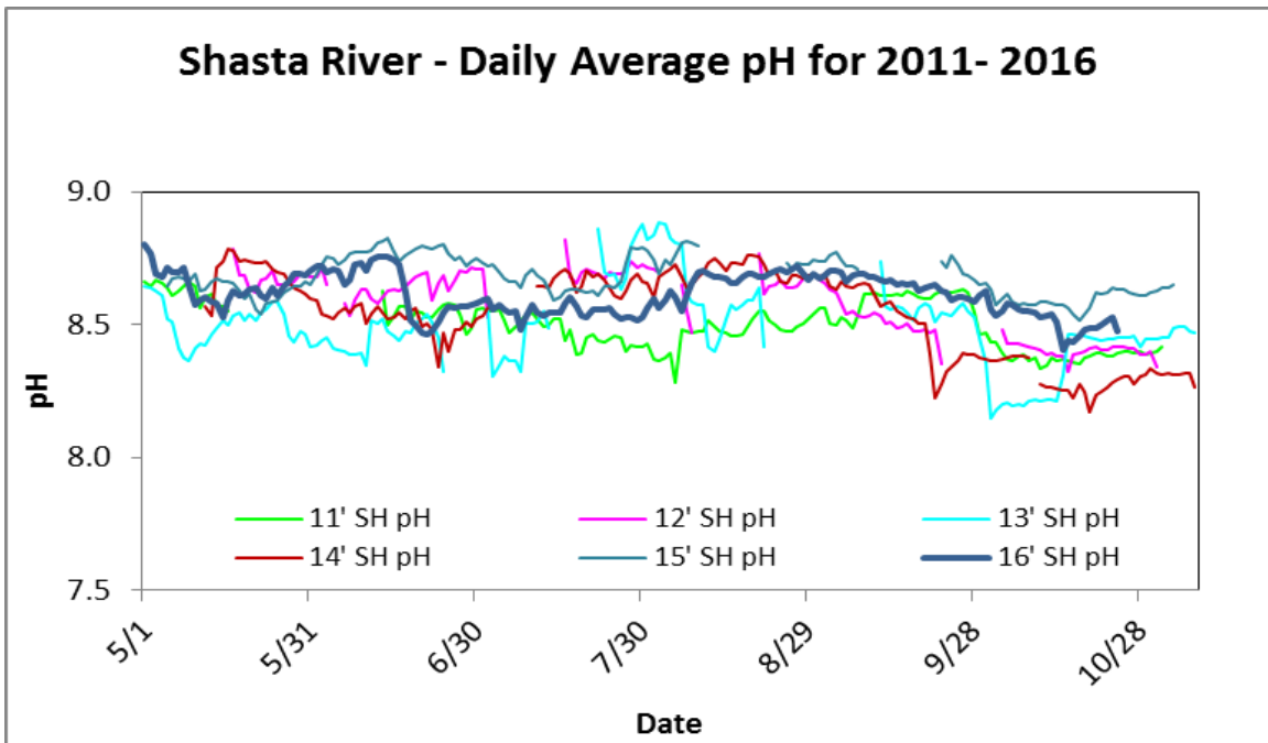
Figure 26. Daily average pH concentrations for the Shasta River from 2011-2016.
