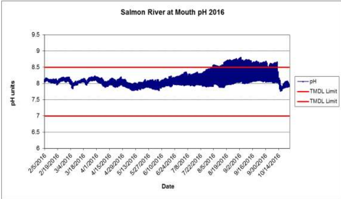
Figure 31. Instantaneous pH readings recorded every 30 minutes for the mouth of the Salmon River (SA) in 2016. The red line indicates the NCRWQCB Basin Plan pH water quality objective for Salmon River, 7 < X < 8.5 .
