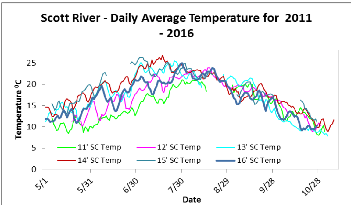
Figure 16. Daily average water temperatures for the Scott River from 2011-2016.
