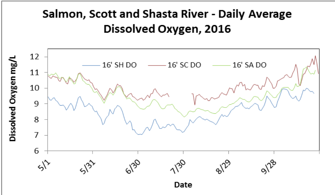
Figure 18. Daily average dissolved oxygen for Salmon, Scott and Shasta River, 2016.
