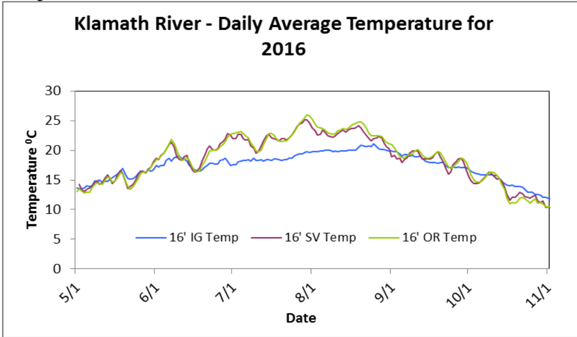
Figure 2. Daily average temperatures for 3 main stem Klamath River sites in 2016: below Iron Gate dam (IG), Seiad Valley (SV), and Orleans (OR).
