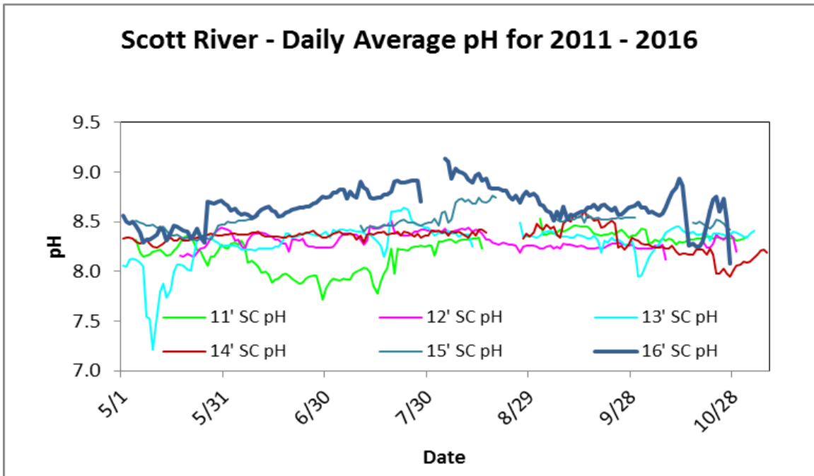
Figure 28. Daily average pH concentrations for the Scott River from 2011-2016.
